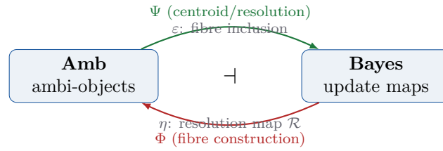
Figure 3: The Ambiguity–Bayes adjunction (Theorem 5.5). The functor \Phi constructs ambi-objects as fibres of Bayesian update maps. The functor \Psi sends each ambi-object to the update map that collapses it to its centroid posterior. Unit \varepsilon is the fibre inclusion; counit \eta is the resolution operator \mathcal{R} .
